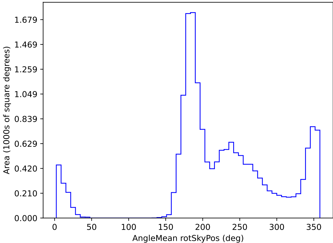
too_elab_r64_d3_gz_v3.4_10yrs WFD z band: AngleMean rotSkyPos
