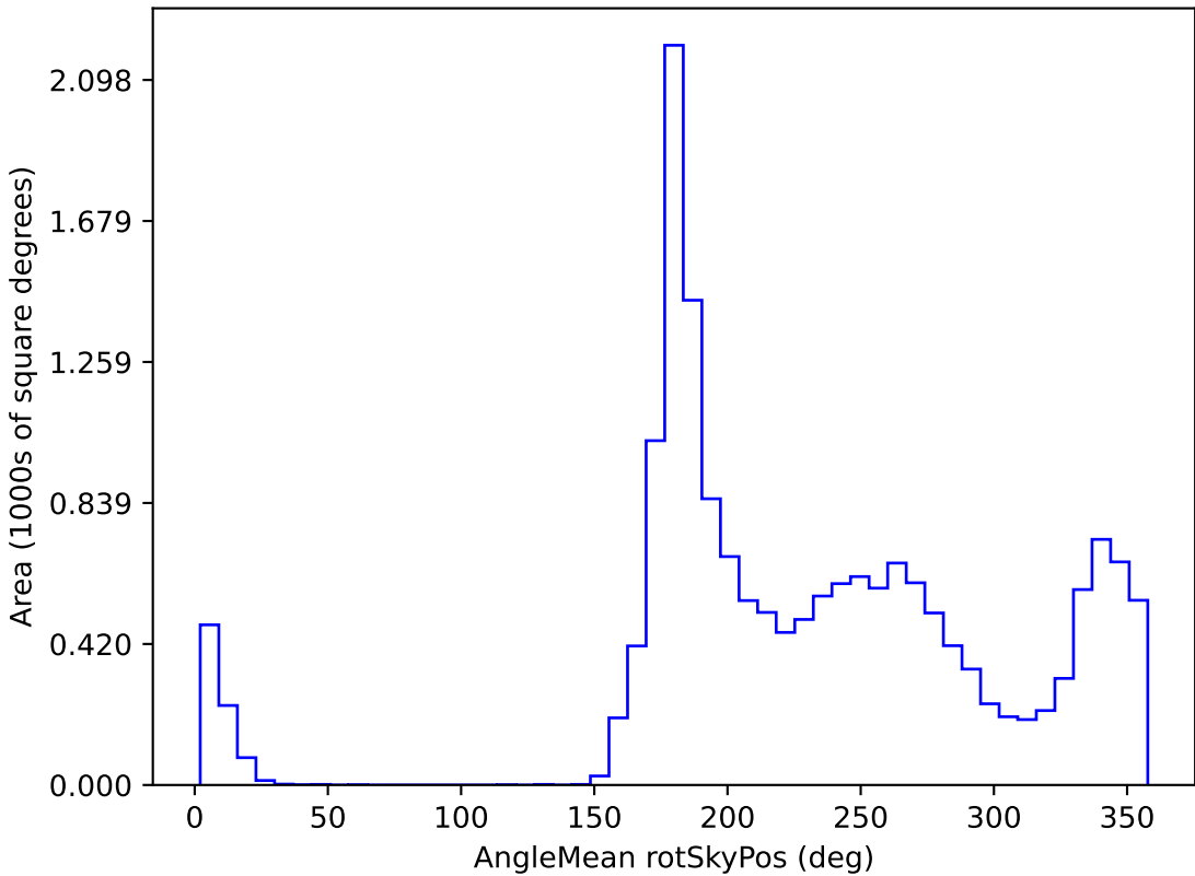
too_elab_r64_d3_gz_v3.4_10yrs WFD y band: AngleMean rotSkyPos
