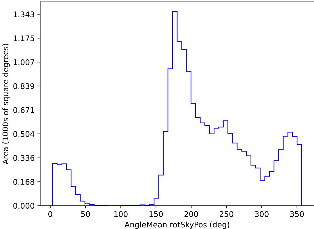
too_elab_r64_d3_gz_v3.4_10yrs WFD u band: AngleMean rotSkyPos
