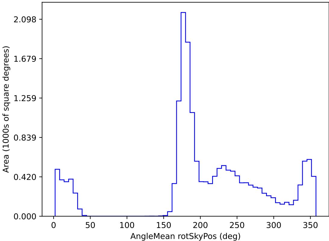
too_elab_r64_d3_gz_v3.4_10yrs WFD r band: AngleMean rotSkyPos
