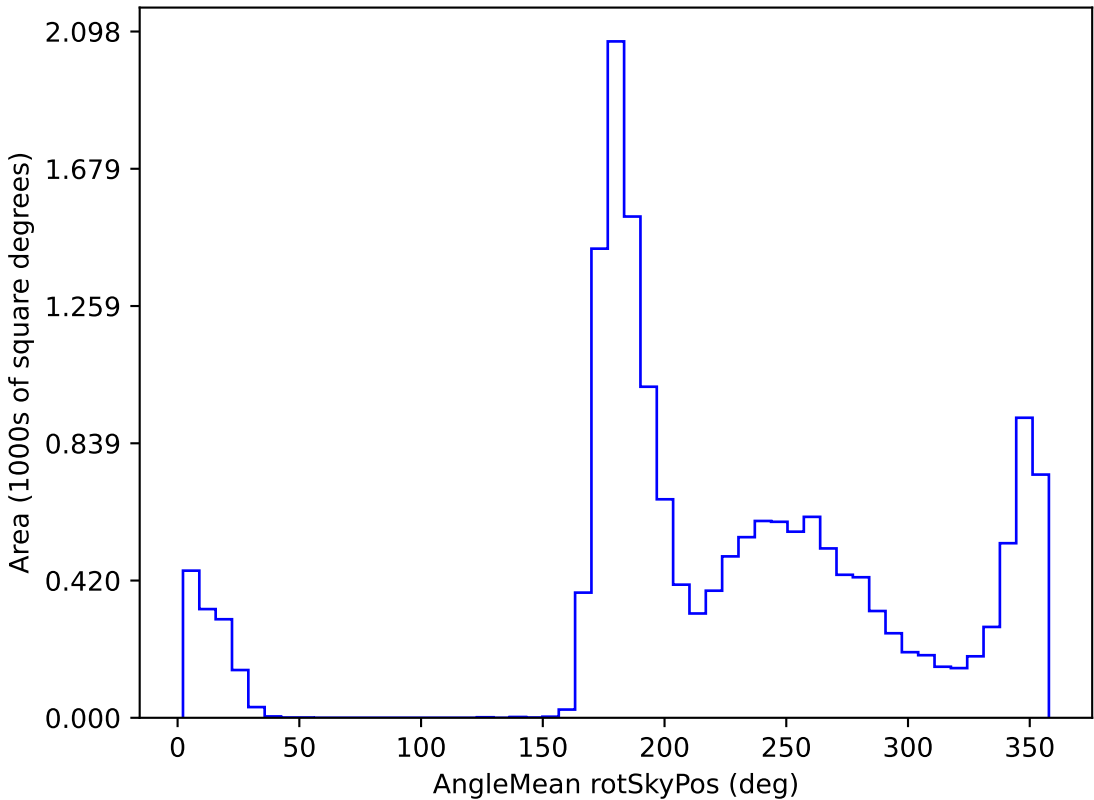
too_elab_r64_d3_gz_v3.4_10yrs WFD i band: AngleMean rotSkyPos
