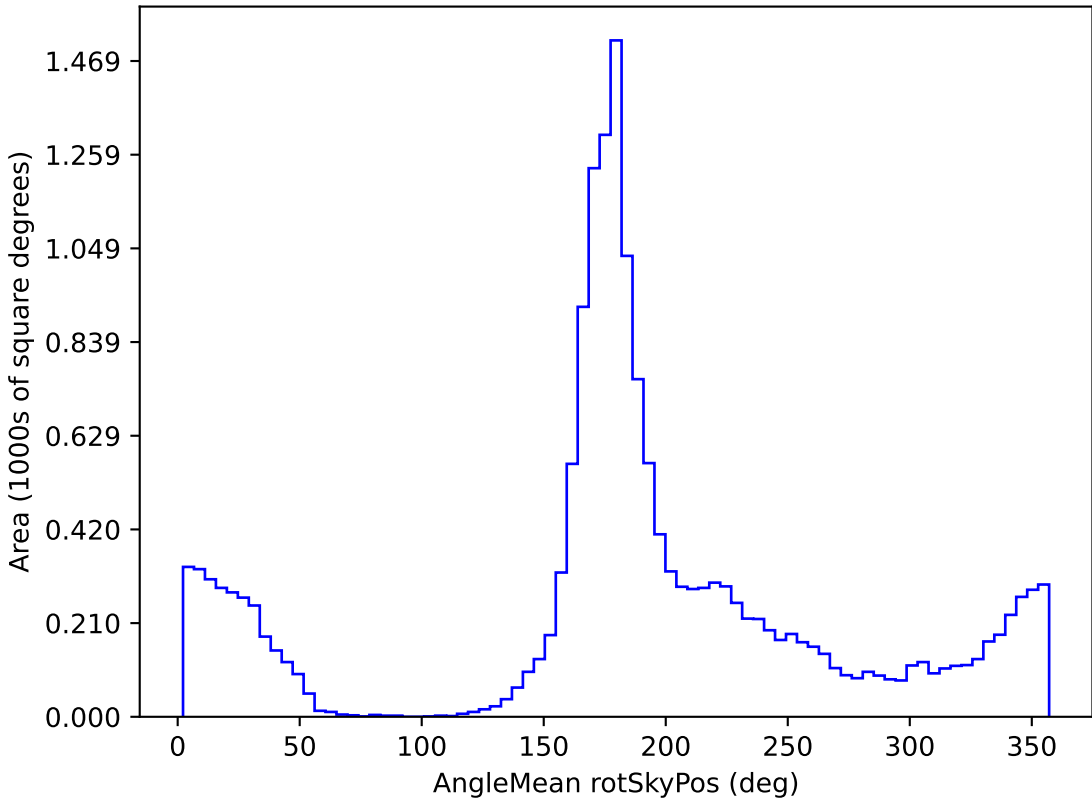
too_elab_r64_d3_gz_v3.4_10yrs WFD g band: AngleMean rotSkyPos
