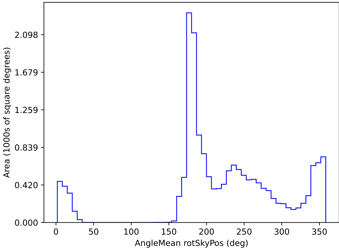
too_elab_r64_d3_gz_v3.4_10yrs WFD all bands: AngleMean rotSkyPos
