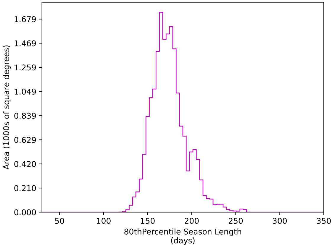
too_elab_r64_d3_gz_v3.4_10yrs WFD z band: 80thPercentile Season Length
