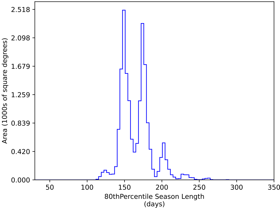
too_elab_r64_d3_gz_v3.4_10yrs WFD y band: 80thPercentile Season Length
