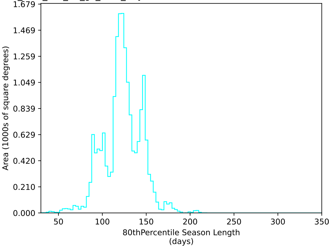
too_elab_r64_d3_gz_v3.4_10yrs WFD u band: 80thPercentile Season Length
