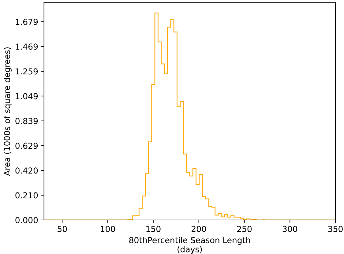
too_elab_r64_d3_gz_v3.4_10yrs WFD r band: 80thPercentile Season Length
