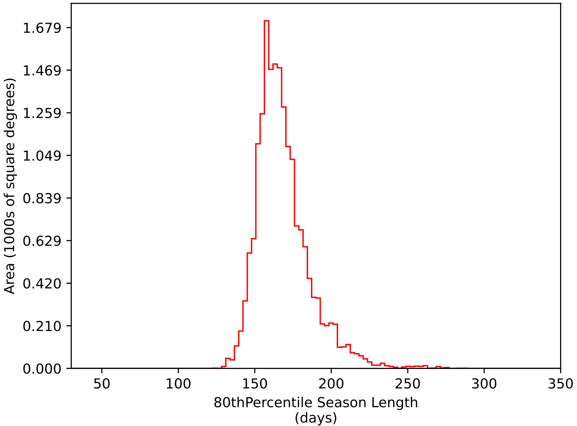
too_elab_r64_d3_gz_v3.4_10yrs WFD i band: 80thPercentile Season Length
