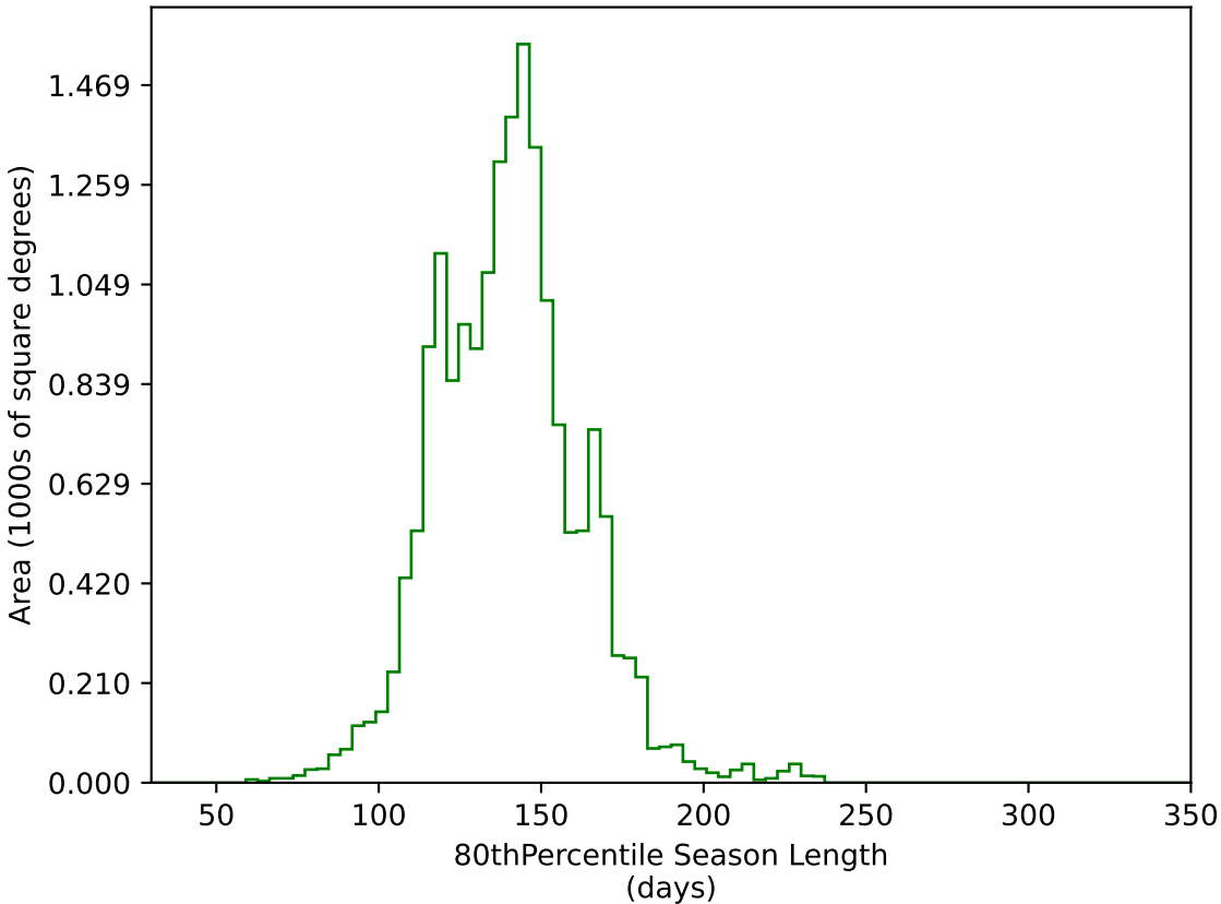
too_elab_r64_d3_gz_v3.4_10yrs WFD g band: 80thPercentile Season Length
