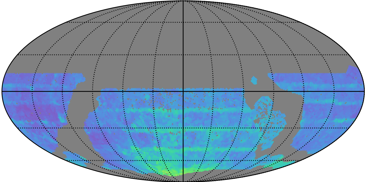
too_elab_r64_d3_gz_v3.4_10yrs WFD all bands: 80thPercentile Season Length
