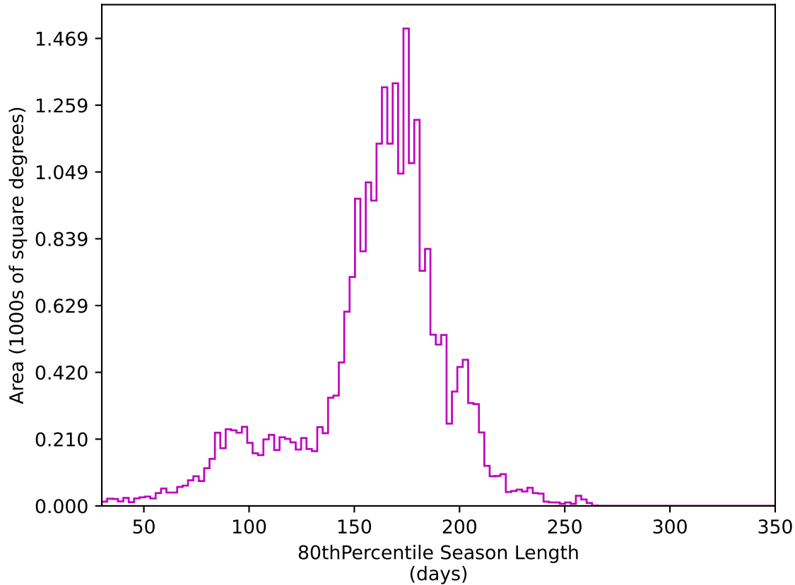
too_elab_r64_d3_gz_v3.4_10yrs All sky z band: 80thPercentile Season Length
