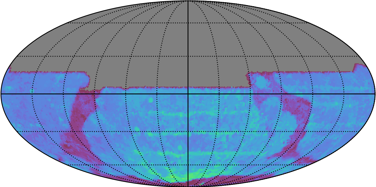
too_elab_r64_d3_gz_v3.4_10yrs All sky y band: 80thPercentile Season Length
