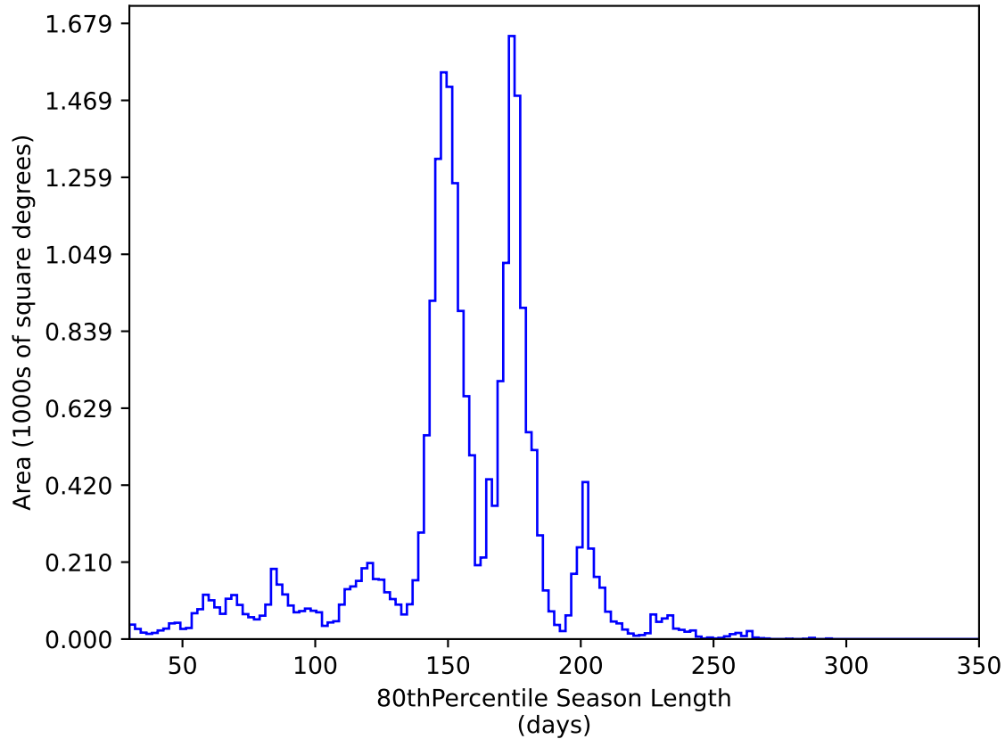
too_elab_r64_d3_gz_v3.4_10yrs All sky y band: 80thPercentile Season Length
