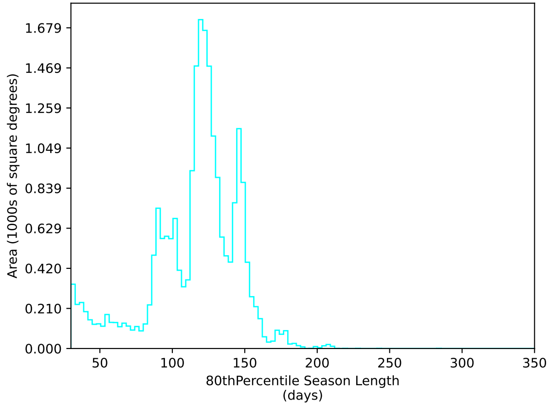
too_elab_r64_d3_gz_v3.4_10yrs All sky u band: 80thPercentile Season Length
