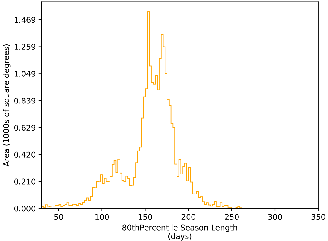
too_elab_r64_d3_gz_v3.4_10yrs All sky r band: 80thPercentile Season Length
