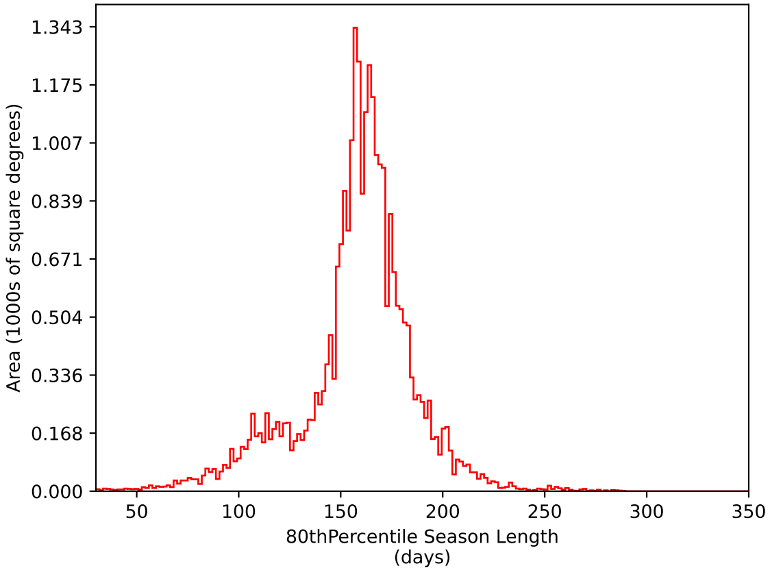
too_elab_r64_d3_gz_v3.4_10yrs All sky i band: 80thPercentile Season Length
