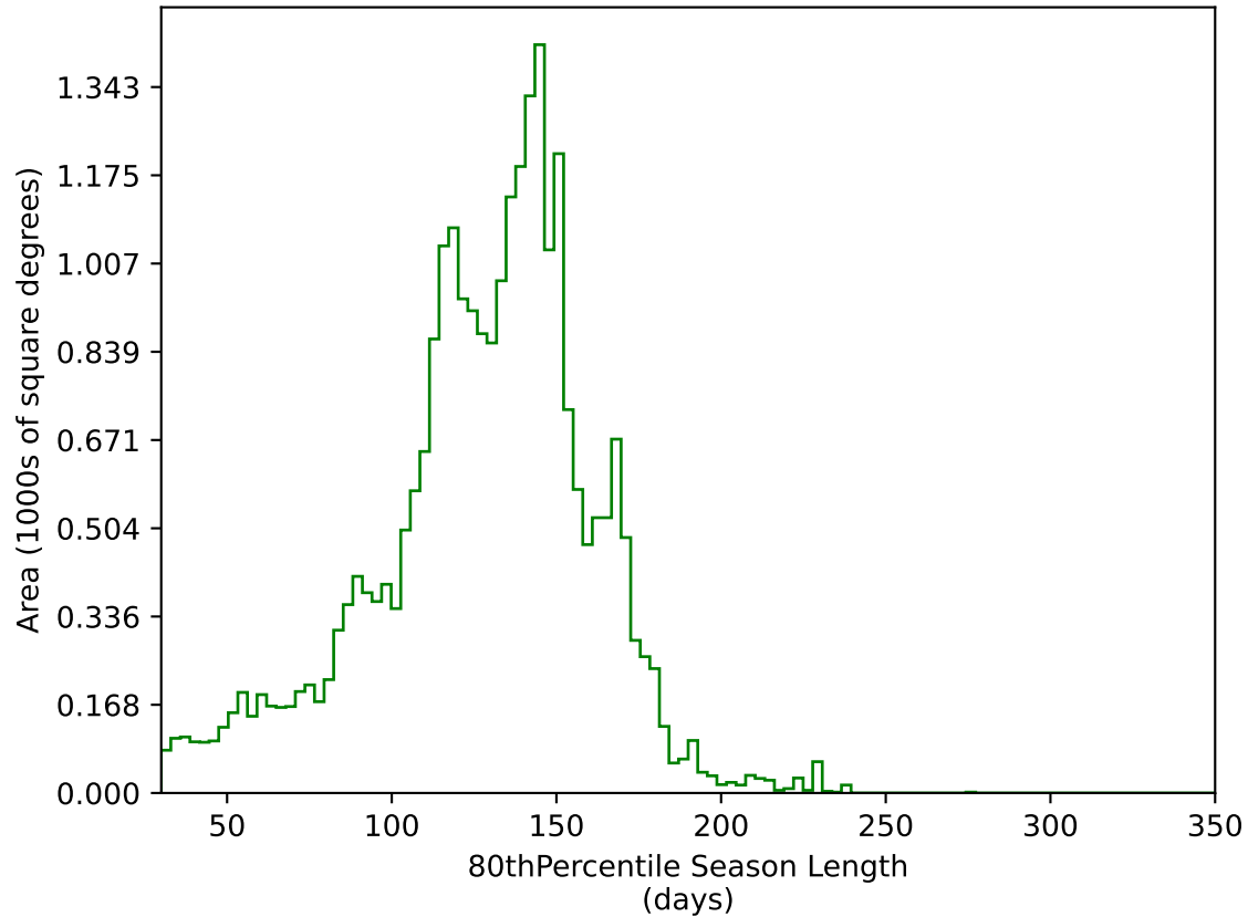
too_elab_r64_d3_gz_v3.4_10yrs All sky g band: 80thPercentile Season Length
