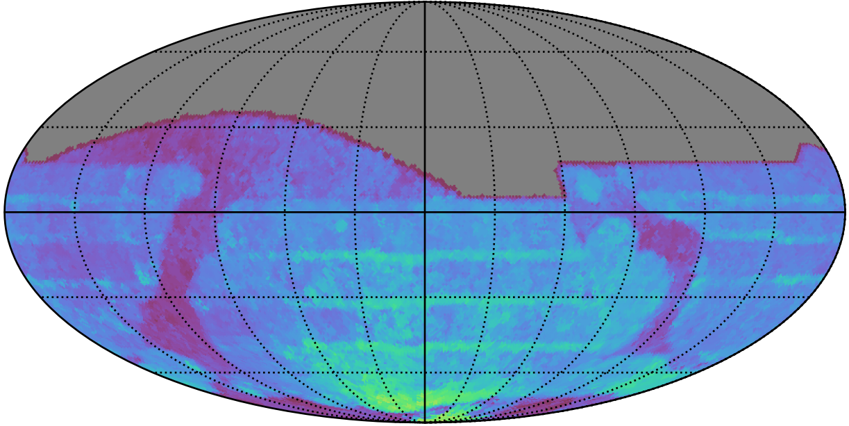
too_elab_r64_d3_gz_v3.4_10yrs All sky all bands: 80thPercentile Season Length
