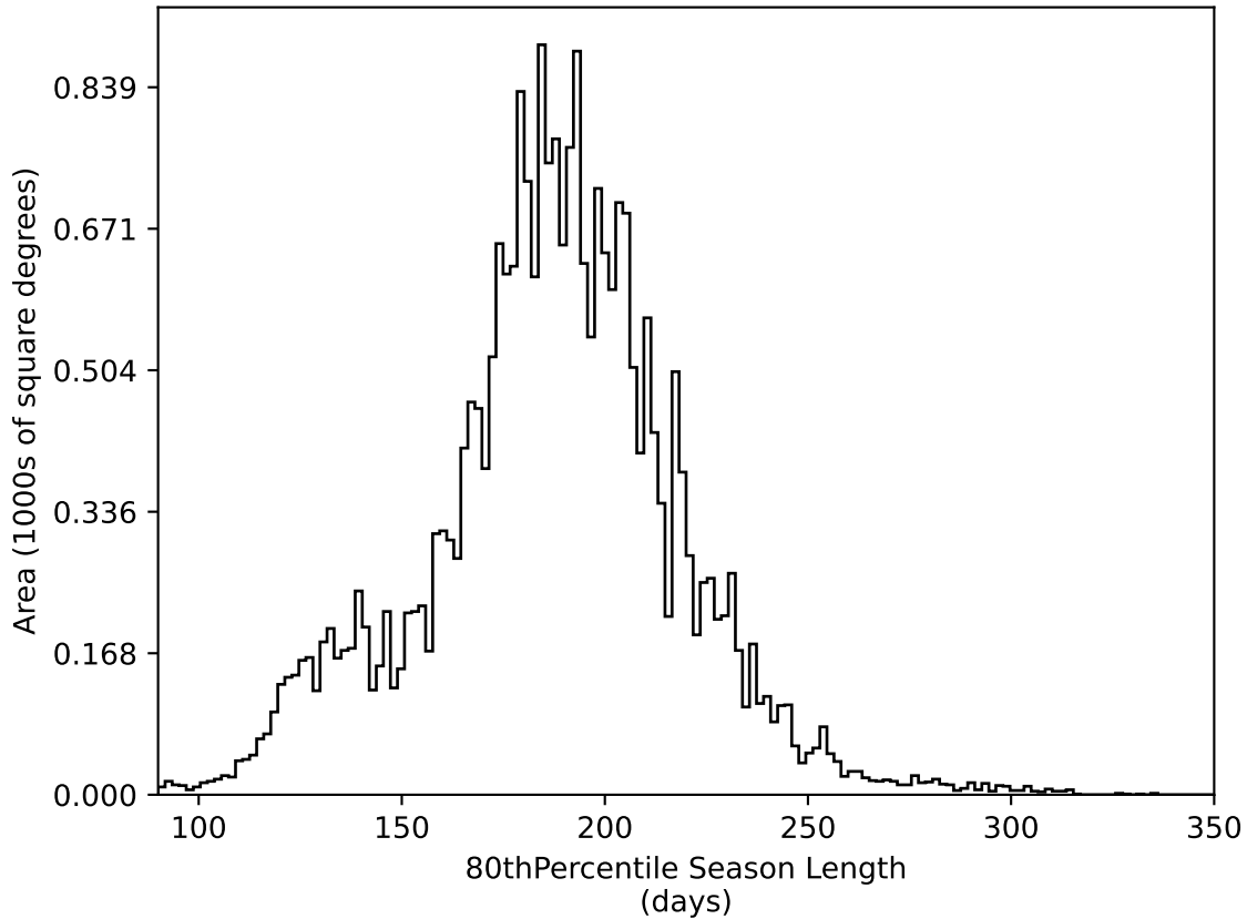
too_elab_r64_d3_gz_v3.4_10yrs All sky all bands: 80thPercentile Season Length
