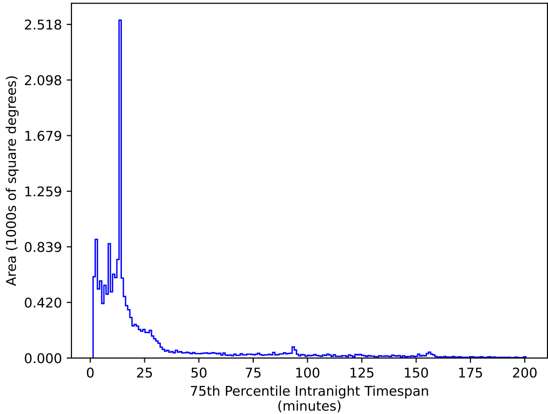
too_elab_r64_d3_gz_v3.4_10yrs WFD z band: 75th Percentile Intranight Timespan
