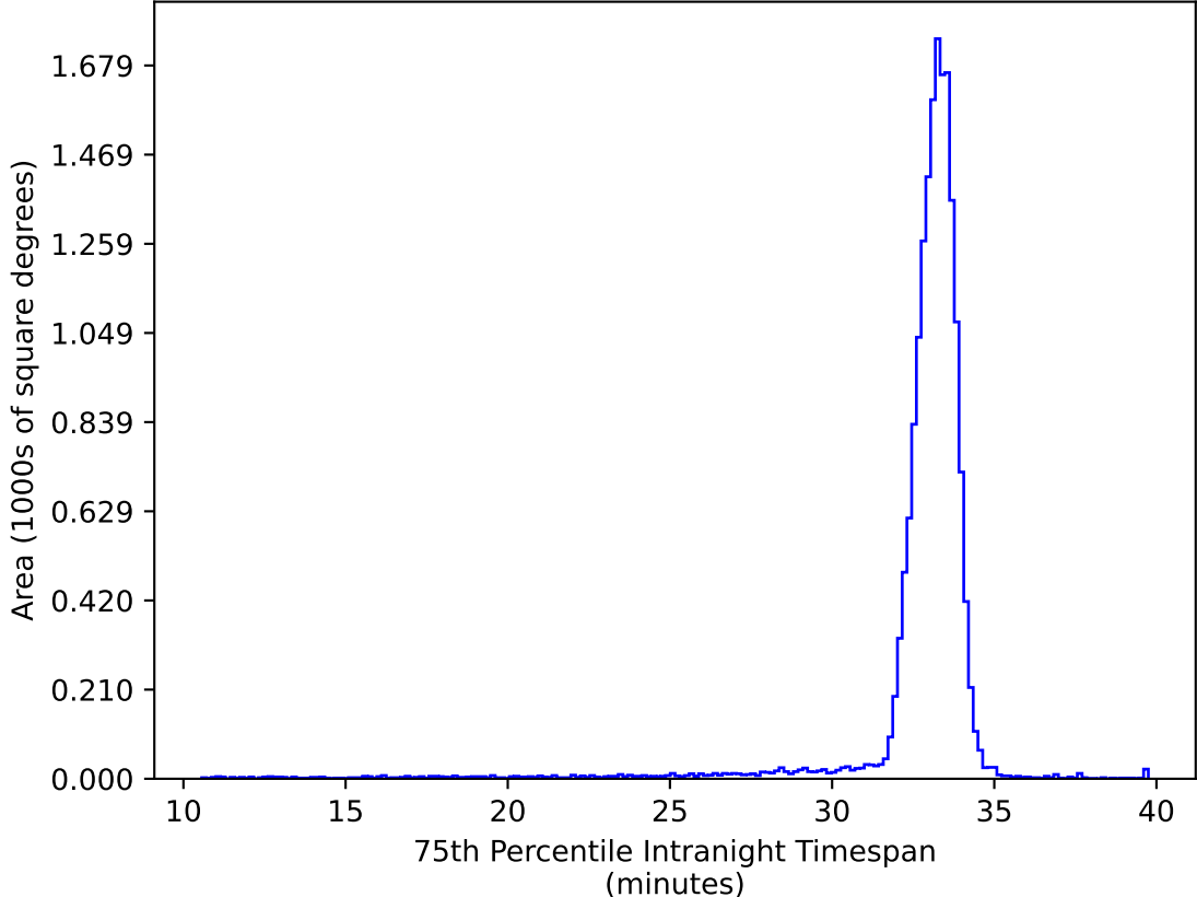
too_elab_r64_d3_gz_v3.4_10yrs WFD ug bands: 75th Percentile Intranight Timespan
