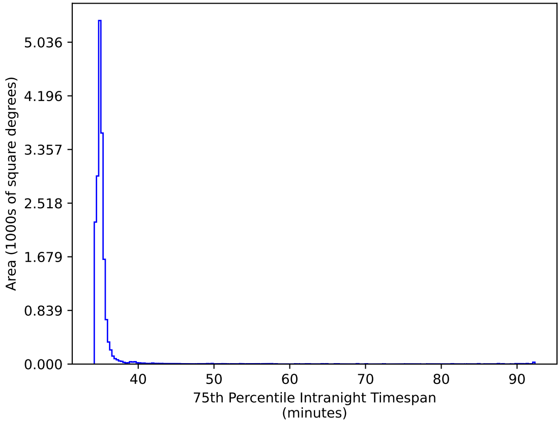
too_elab_r64_d3_gz_v3.4_10yrs WFD ri bands: 75th Percentile Intranight Timespan
