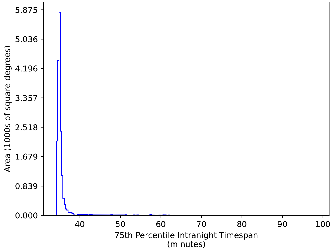
too_elab_r64_d3_gz_v3.4_10yrs WFD gr bands: 75th Percentile Intranight Timespan
