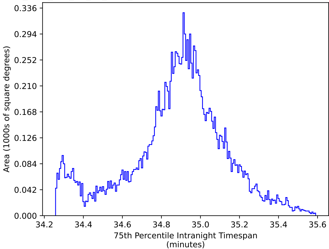
too_elab_r64_d3_gz_v3.4_10yrs WFD: 75th Percentile Intranight Timespan
