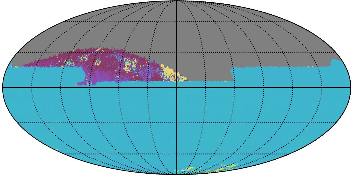
too_elab_r64_d3_gz_v3.4_10yrs All sky zy bands: 75th Percentile Intranight Timespan
