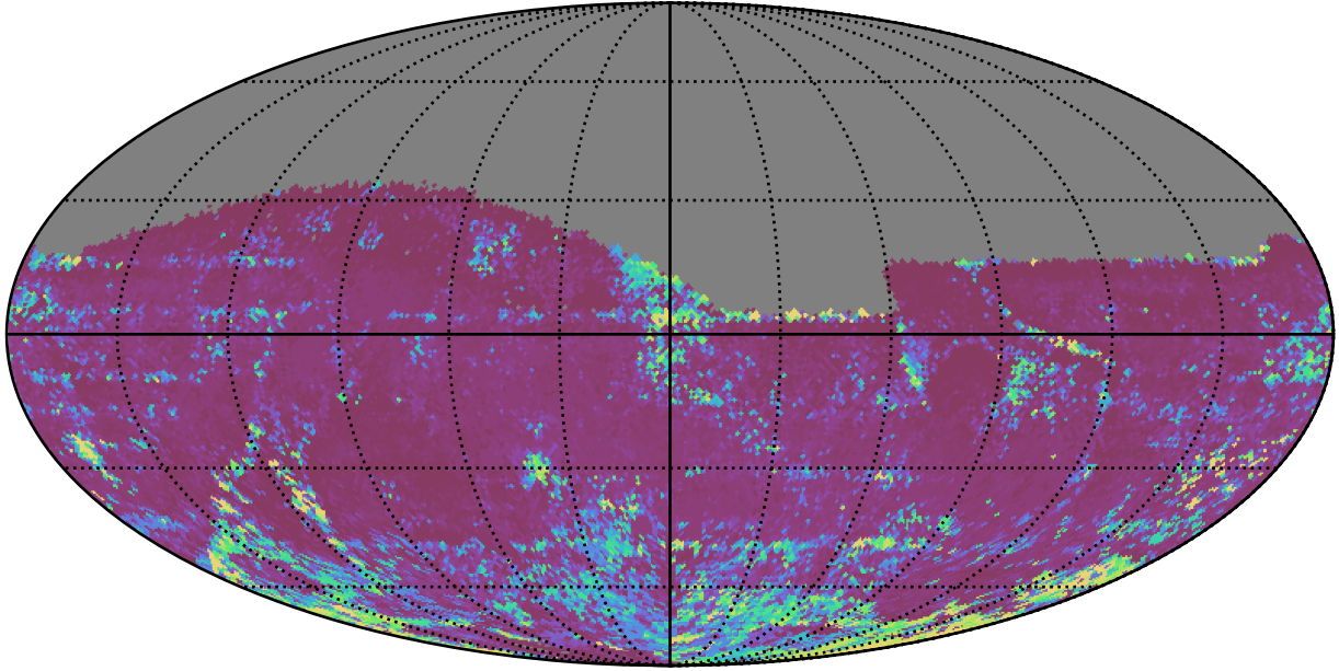
too_elab_r64_d3_gz_v3.4_10yrs All sky z band: 75th Percentile Intranight Timespan
