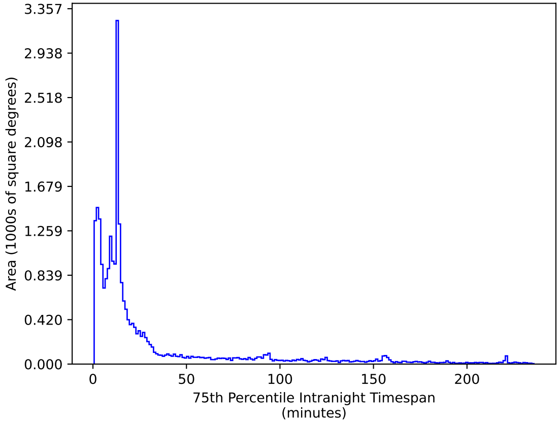
too_elab_r64_d3_gz_v3.4_10yrs All sky z band: 75th Percentile Intranight Timespan
