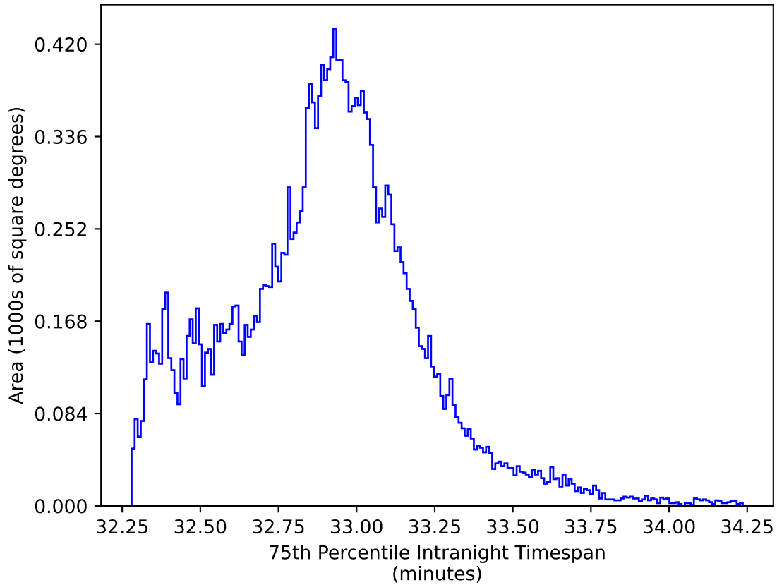
too_elab_r64_d3_gz_v3.4_10yrs All sky y band: 75th Percentile Intranight Timespan
