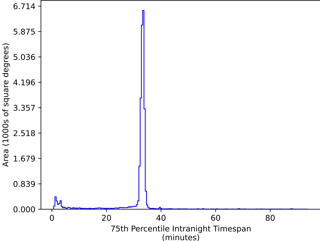
too_elab_r64_d3_gz_v3.4_10yrs All sky ug bands: 75th Percentile Intranight Timespan
