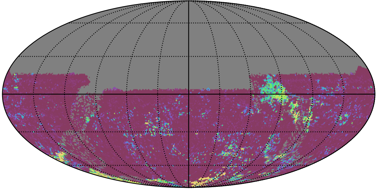
too_elab_r64_d3_gz_v3.4_10yrs All sky u band: 75th Percentile Intranight Timespan
