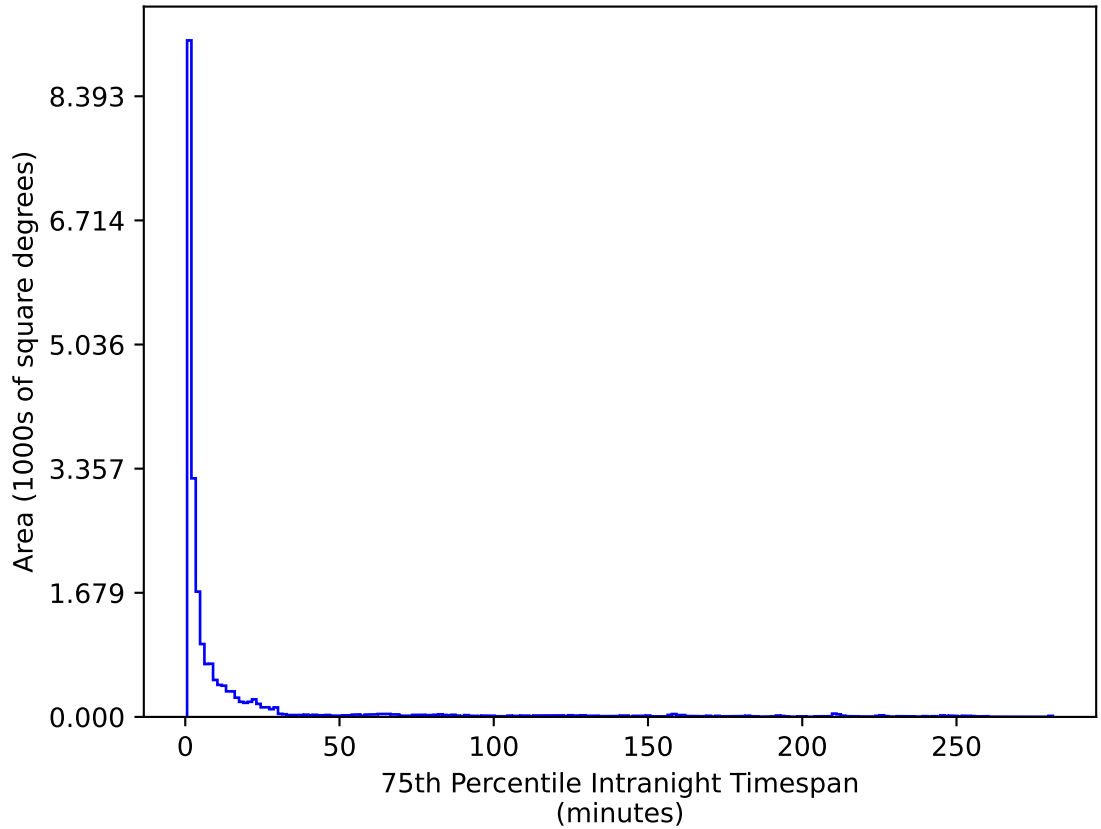
too_elab_r64_d3_gz_v3.4_10yrs All sky u band: 75th Percentile Intranight Timespan
