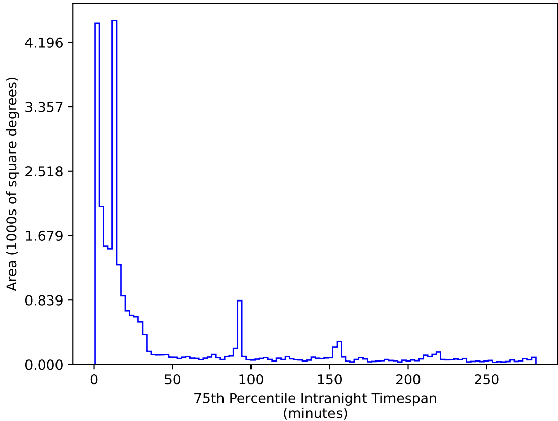
too_elab_r64_d3_gz_v3.4_10yrs All sky r band: 75th Percentile Intranight Timespan
