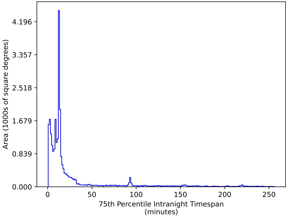
too_elab_r64_d3_gz_v3.4_10yrs All sky i band: 75th Percentile Intranight Timespan
