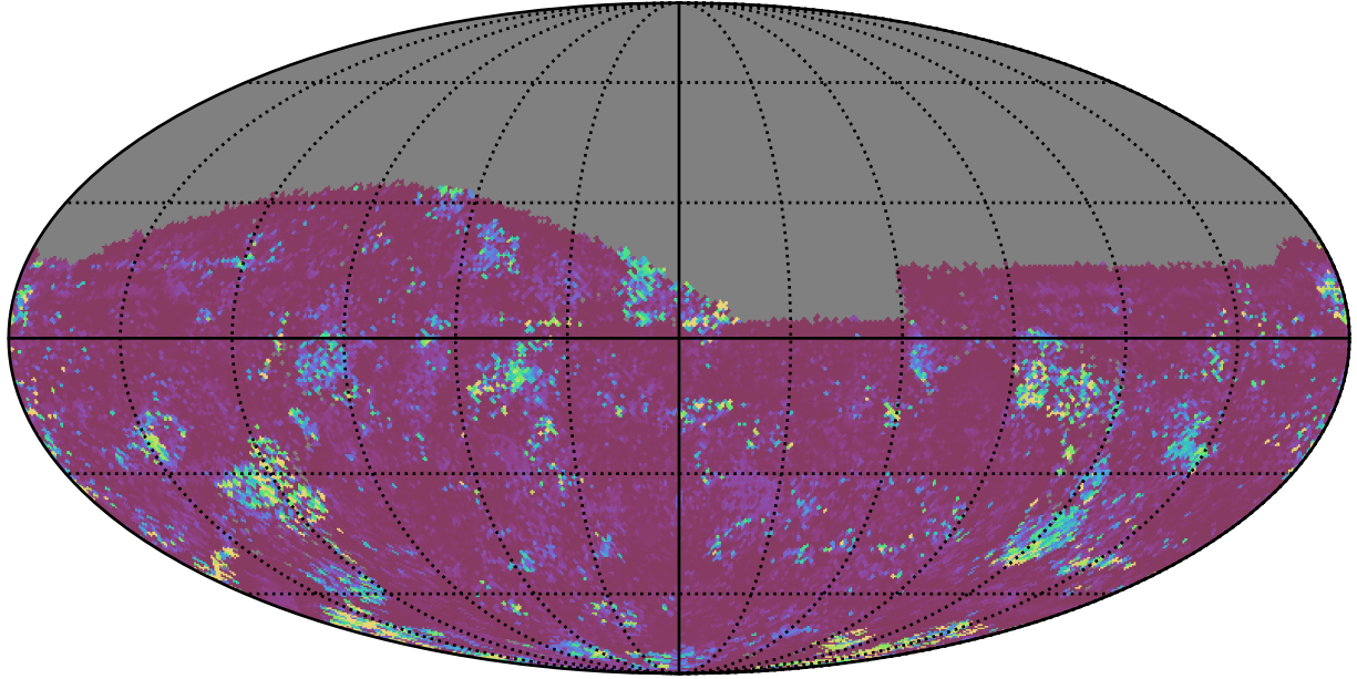
too_elab_r64_d3_gz_v3.4_10yrs All sky g band: 75th Percentile Intranight Timespan
