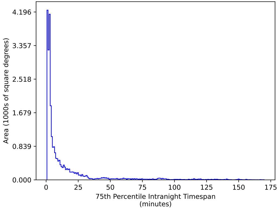
too_elab_r64_d3_gz_v3.4_10yrs All sky g band: 75th Percentile Intranight Timespan
