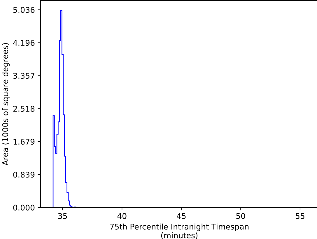
too_elab_r64_d3_gz_v3.4_10yrs All sky all bands: 75th Percentile Intranight Timespan
