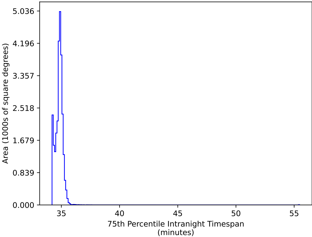
too_elab_r64_d3_gz_v3.4_10yrs All sky: 75th Percentile Intranight Timespan
