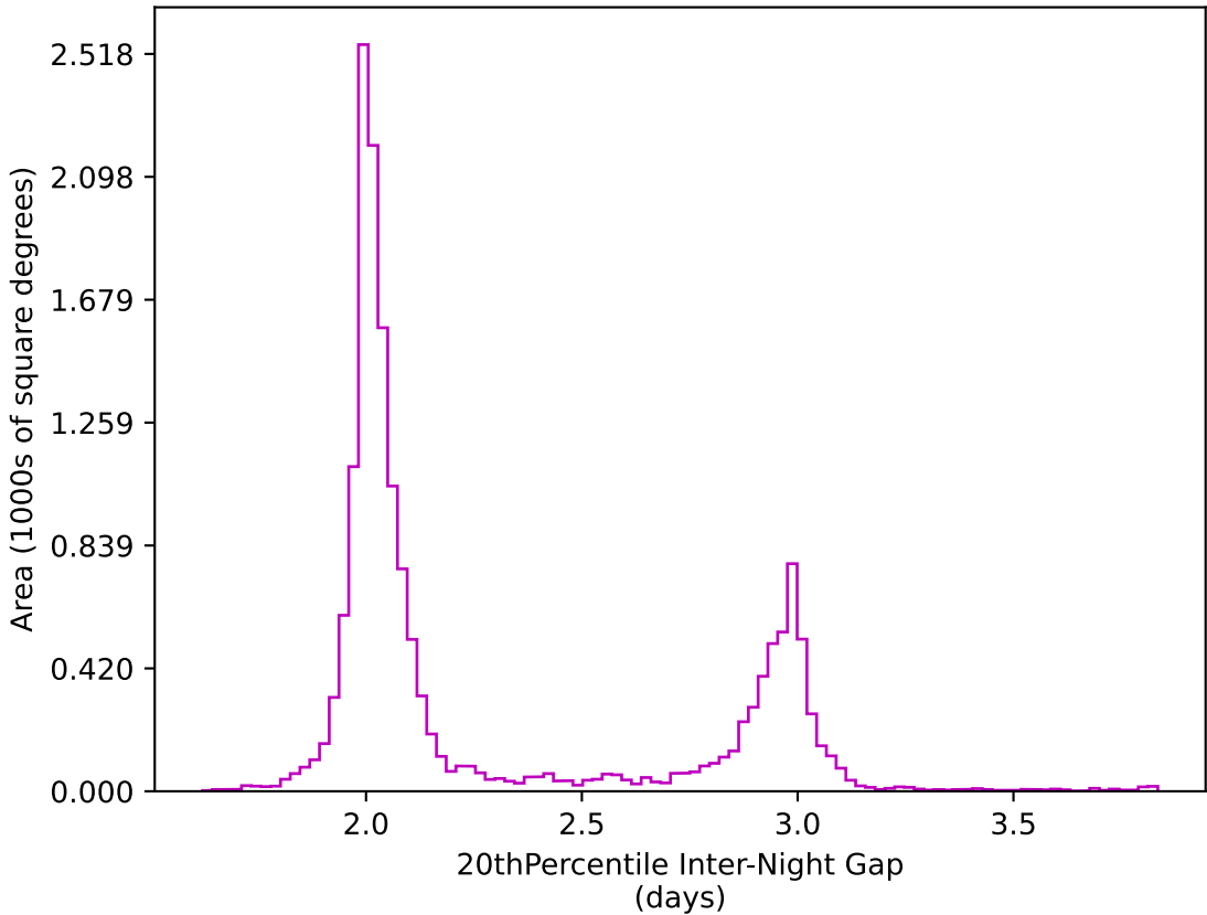
too_elab_r64_d3_gz_v3.4_10yrs WFD z band: 20thPercentile Inter-Night Gap
