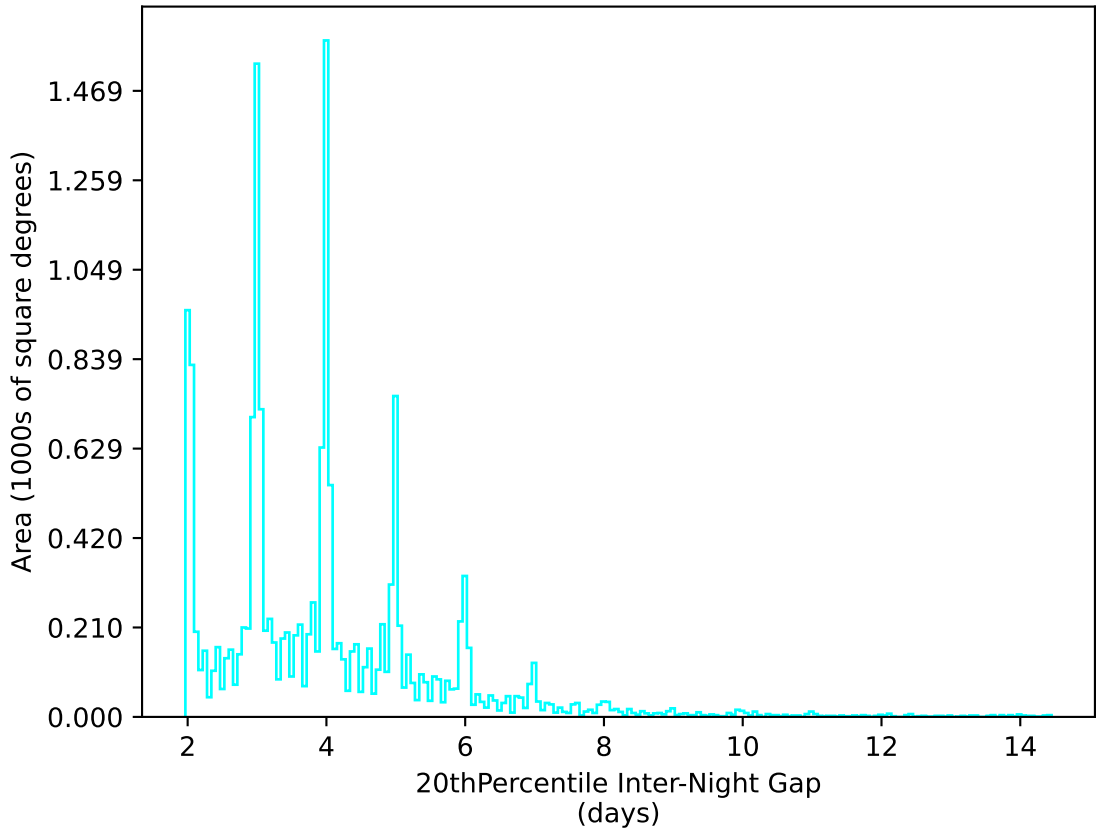
too_elab_r64_d3_gz_v3.4_10yrs WFD u band: 20thPercentile Inter-Night Gap
