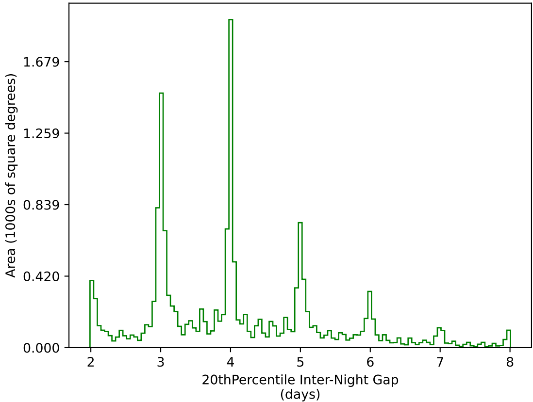
too_elab_r64_d3_gz_v3.4_10yrs WFD g band: 20thPercentile Inter-Night Gap
