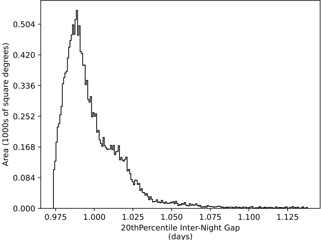
too_elab_r64_d3_gz_v3.4_10yrs WFD all bands: 20thPercentile Inter-Night Gap
