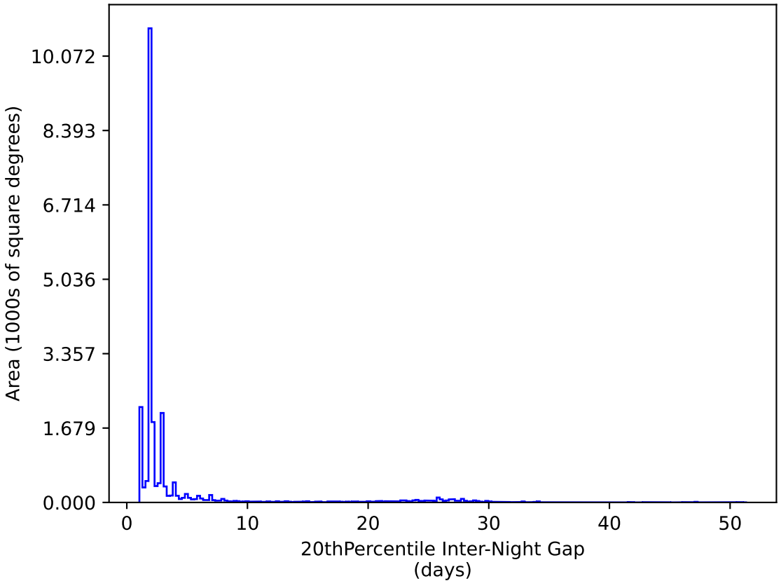
too_elab_r64_d3_gz_v3.4_10yrs All sky y band: 20thPercentile Inter-Night Gap
