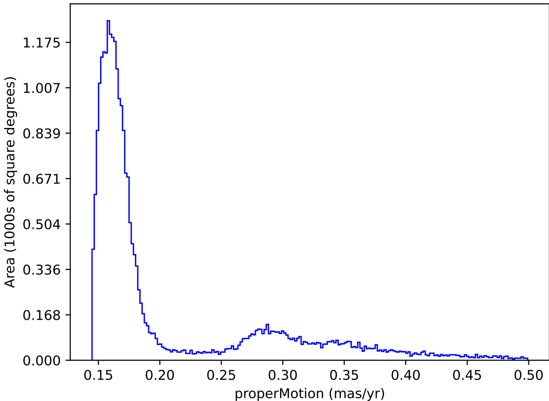
too_elab_r64_d3_gz_v3.4_10yrs : properMotion
