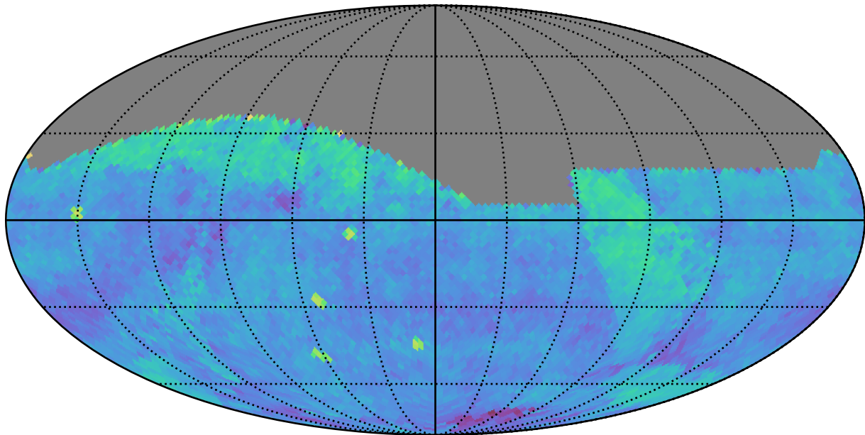
too_elab_r64_d3_gz_v3.4_10yrs (g or r or i): PairFraction
