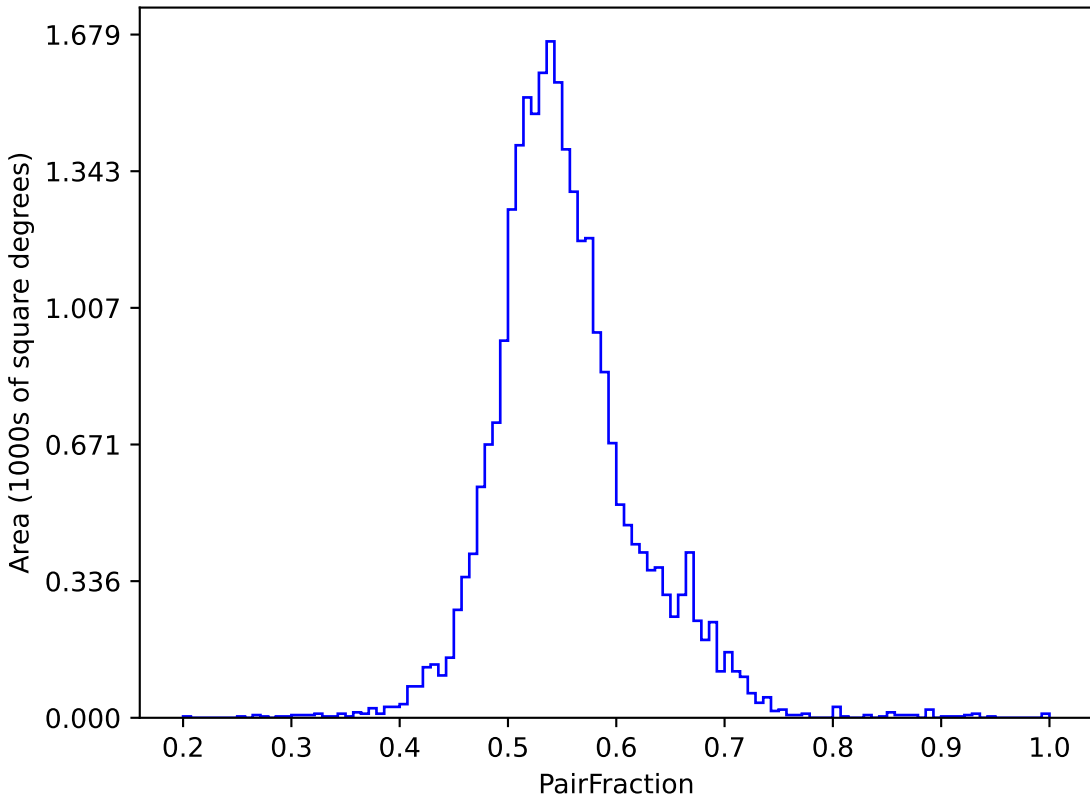
too_elab_r64_d3_gz_v3.4_10yrs (g or r or i): PairFraction
