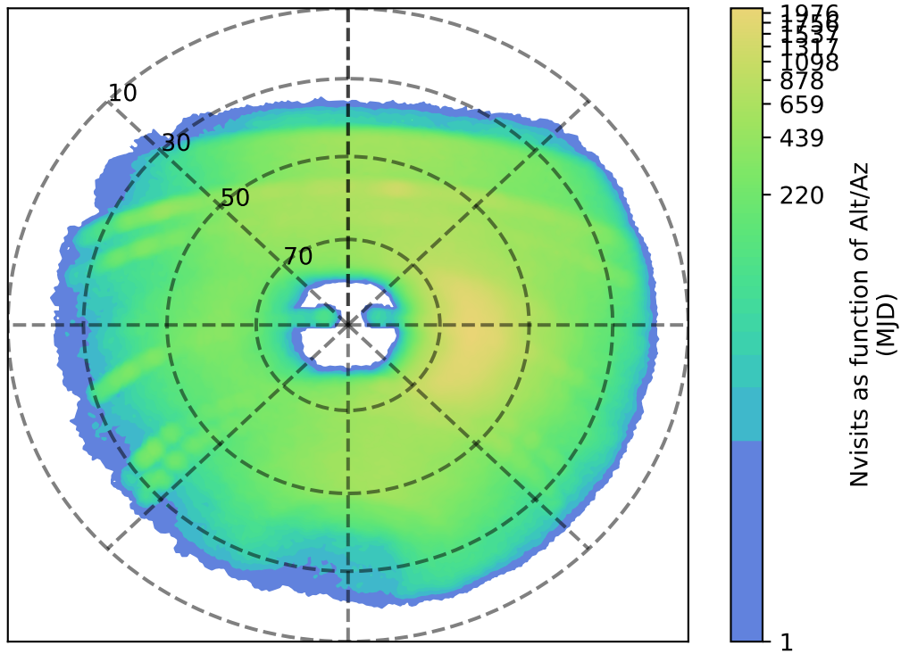
too_elab_r64_d3_gz_v3.4_10yrs y: Nvisits as function of Alt/Az
